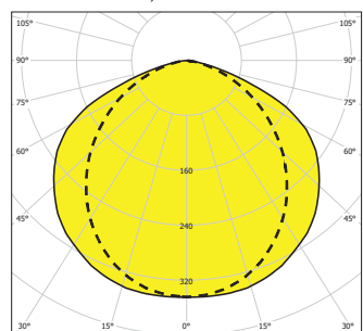
SALUKA-N-LED-236, IP66
